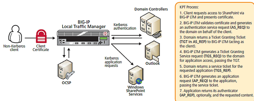
Kerberos protocol transition on BIG-IP LTM.
