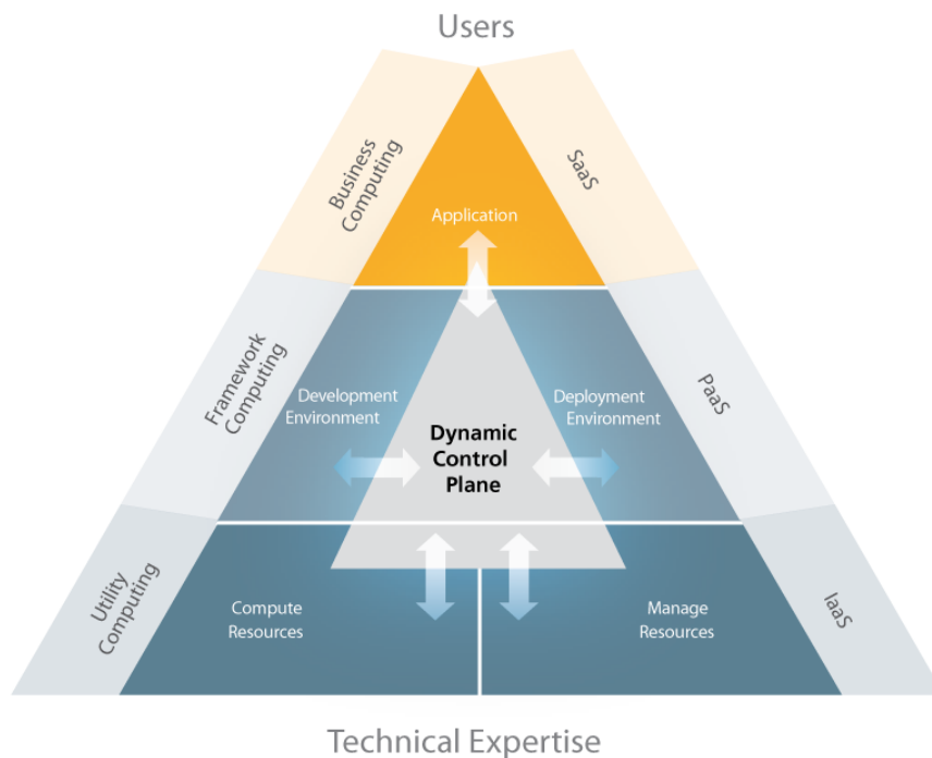
Figure 1. Cloud architecture
