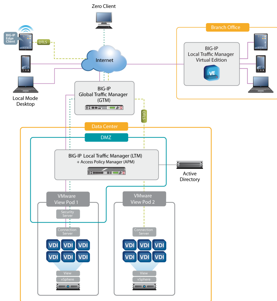
Figure 1: The F5 BIG-IP system and VMware Horizon View topology.
