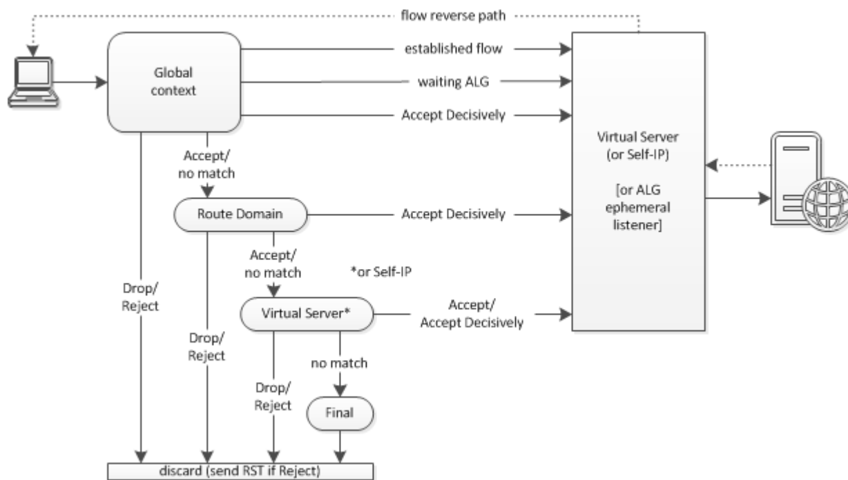
Figure 3: The Firewall Policy Context Hierarchy (omits management-port context)
