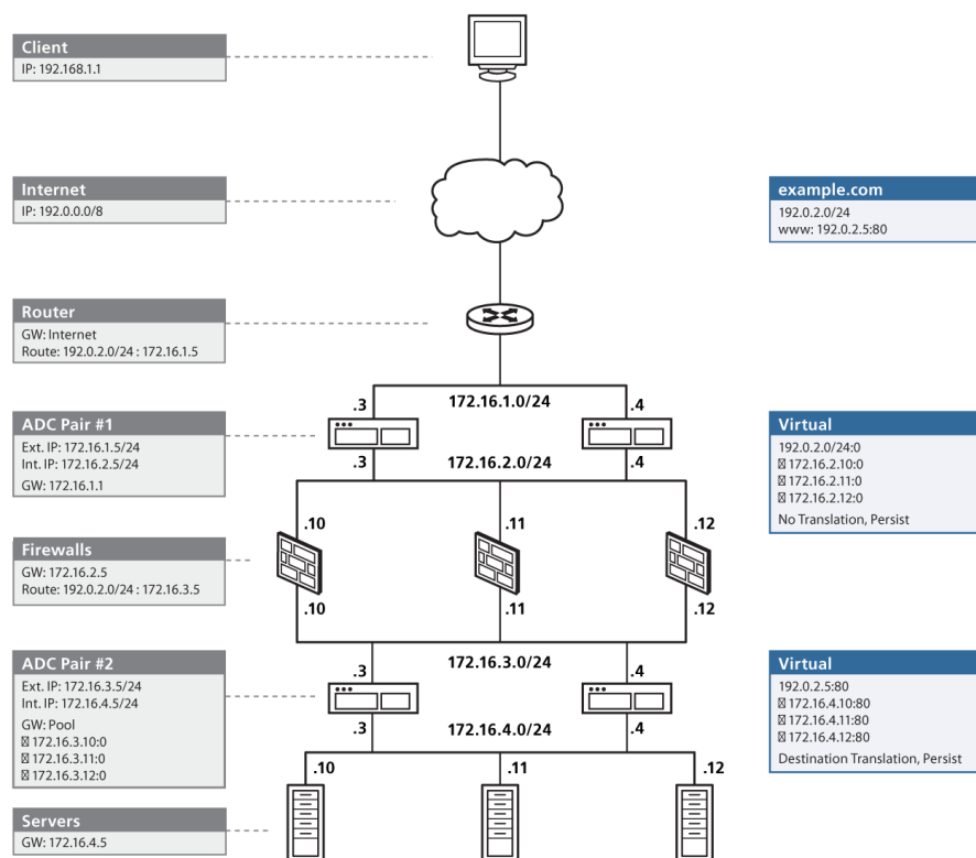
Figure 1. A basic firewall sandwich design
