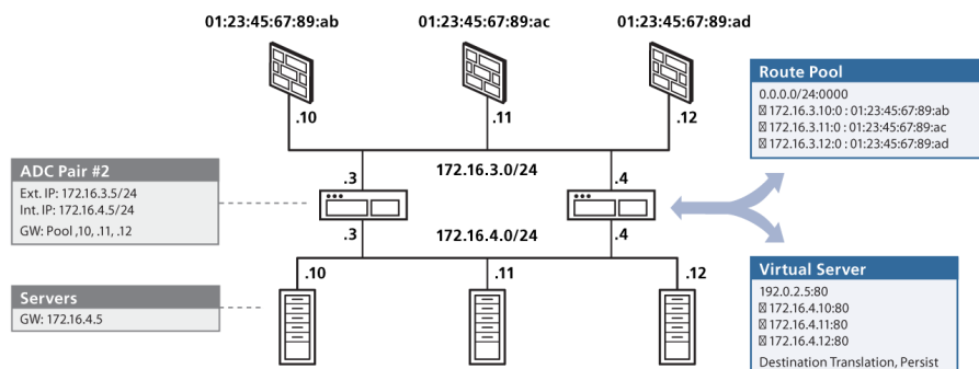
Figure 2. Last-hop return routing by MAC
