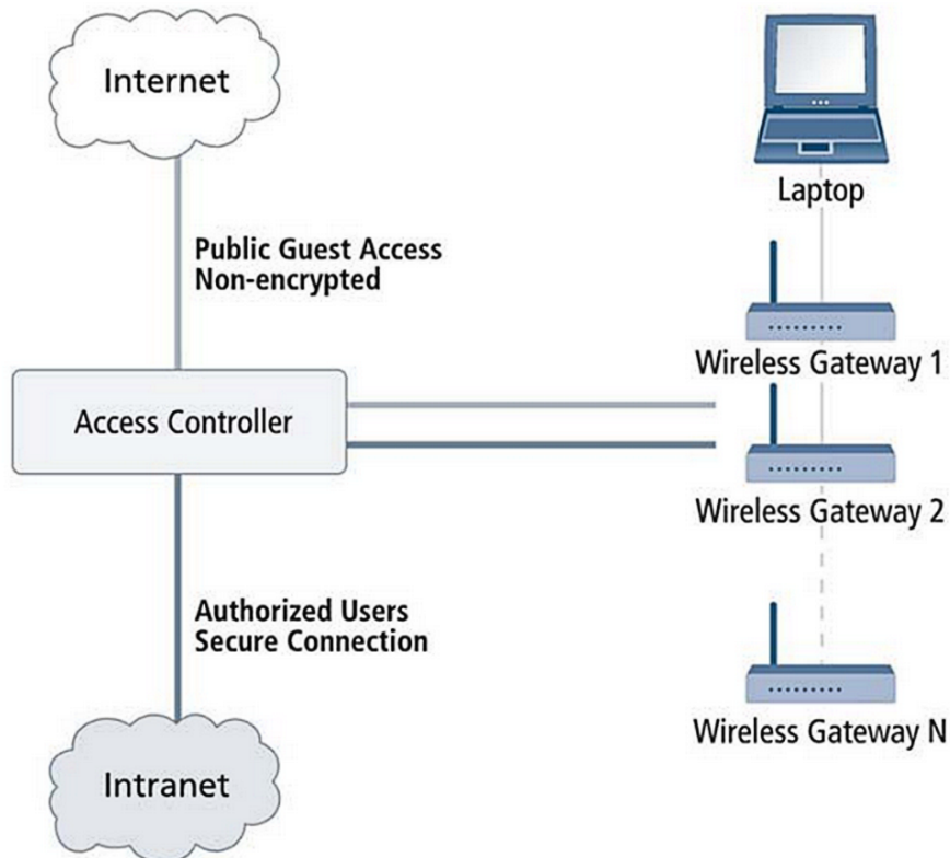
Figure 1: Wireless Access
